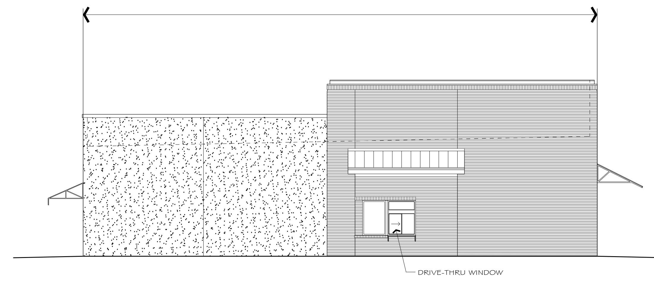
3 WEST ELEVATION
